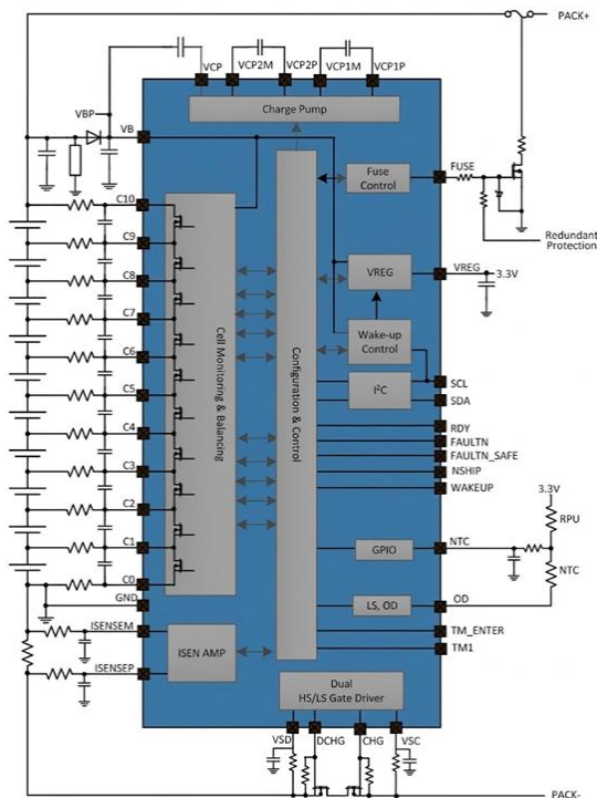
Figure. The L9962 measures individual cell voltages on a continuous cycle with programmable loop time and activates balancing and cell protection upon detecting overvoltage or undervoltage. In addition, plausibility checking compares the total stack voltage with the number of cells. While ensuring cell voltages remain tightly aligned, the L9962 maintains voltage-measurement accuracy across the full operating-temperature range.
